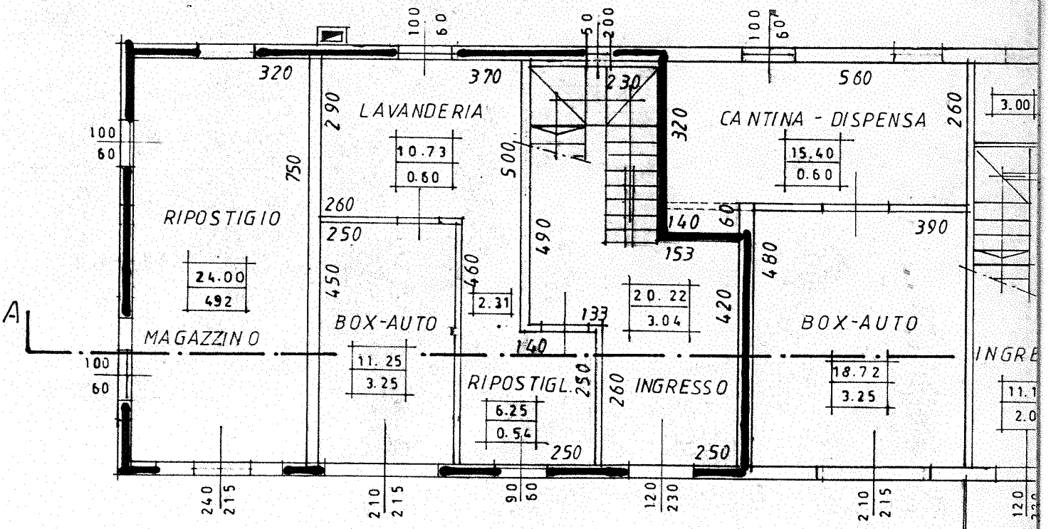
PIANO TERRA
